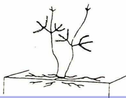
Streptoverticillium
