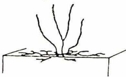
Actinopolyspora
