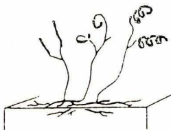
Streptomyces
