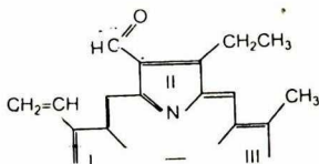
Chlorophin b
