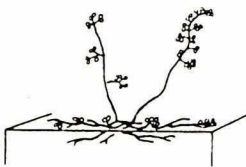
Thermomonospora
