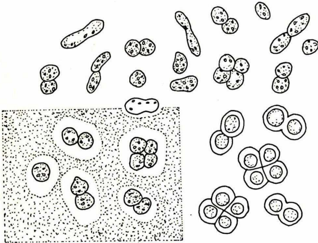
Azotobacter
