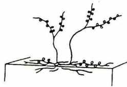
Thermoactinomyces
