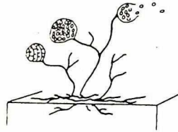
Streptosporangium
