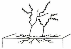
Nocardiopsis
