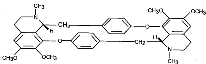
Cycleanin
