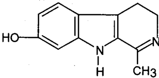
Harmalol
