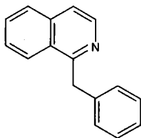
Kiểu benzyloisoquinolin
