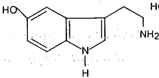
Serotonin
