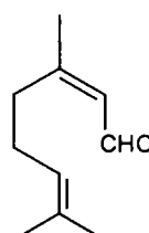
Citral b
