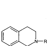
Kiểu tetrahydroisoquinolin
