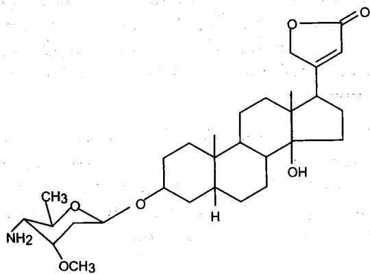
Nor - mitiphyllin
