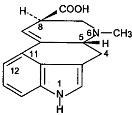
Acid lysergic
