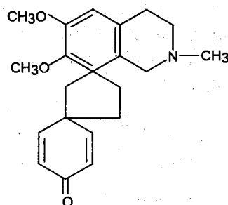
Pro-nuciferin
