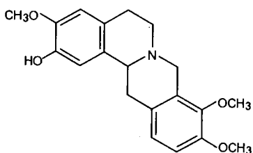
Tetrahydrocolumbamin (isocorypalmin)
