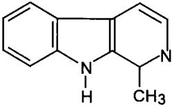
Harman
