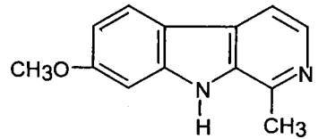
Harmin
