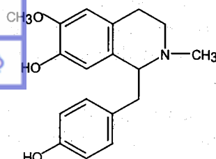
Metyl coclaurin
