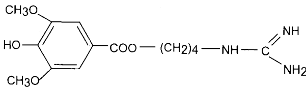
Leonurin
