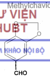
Aldehyd cinamic
