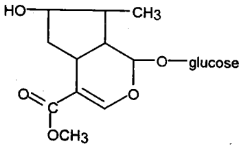
Loganin
