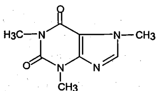
Cafein
