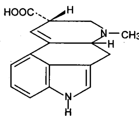
Acid isolysergic
