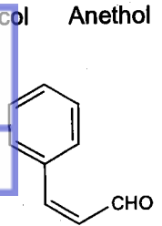
Anethol
