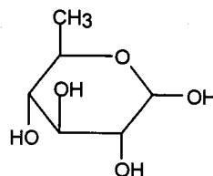
Quinovose
