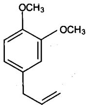
Methyleugenol
