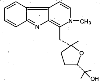
Isochrysocticin
