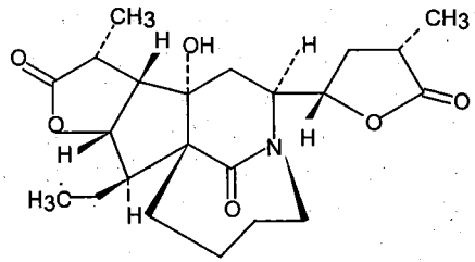
Tuberostemoninol
