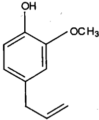
Eugenol
